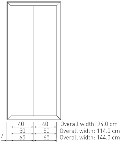
Layout of combination panels
