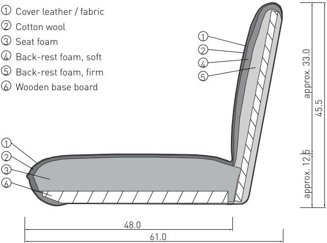
Upholstered bench design
