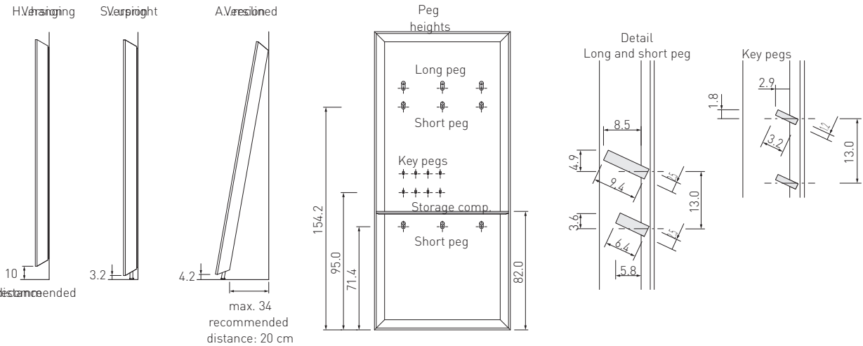
Type and dimensions of Haiku wall panel
