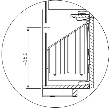
Detail view of wiring for charging station Qi
