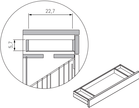
Detail view of drawer (internal dimensions)
