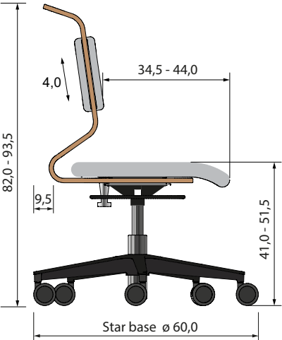
Seat width: 44.5 cm
