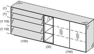
cubus pure Sideboard 72
